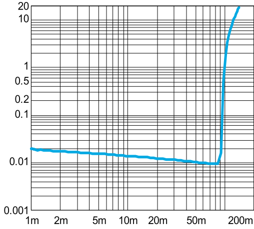
THD+N vs. Output Power SE mode, 5V, 320ohm, f=1 kHz
