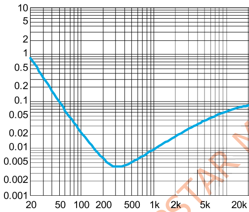
THD+N vs. Frequency SE mode, 6V, 320ohm, Po=70mW
