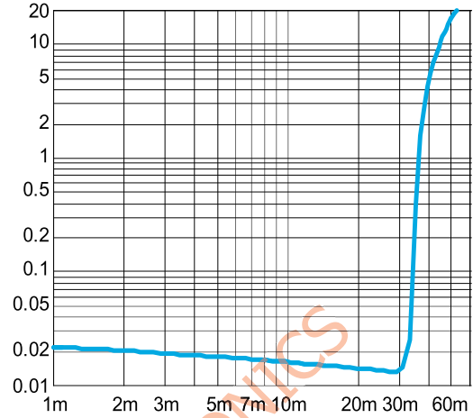
THD+N vs. Output Power SE mode, 3V, 320ohm, f=1 kHz
