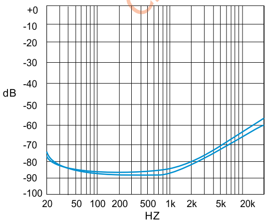
PSRR vs. Freq SE mode, 6V, 320ohm, 200mVpp Input terminated
