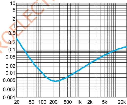
THD+N vs. Frequency SE mode, 3V, 320ohm, Po=20mW
