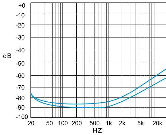
PSRR vs. Freq SE mode, 3V, 320ohm, 200mVpp Input terminated
