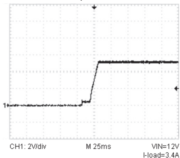
Start-up Waveform
