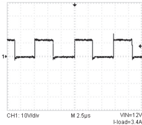
Start-up Waveform
