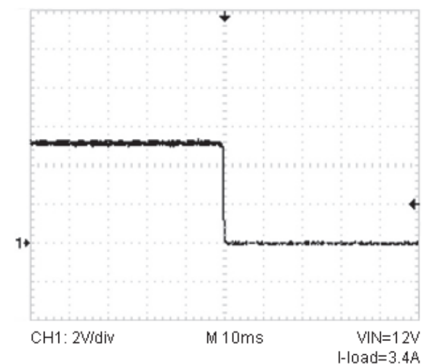
Shutdown Waveform
